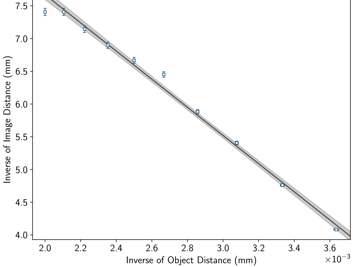
Inverse of Image Distance (mm) vs. Inverse of Object Distance (mm)
