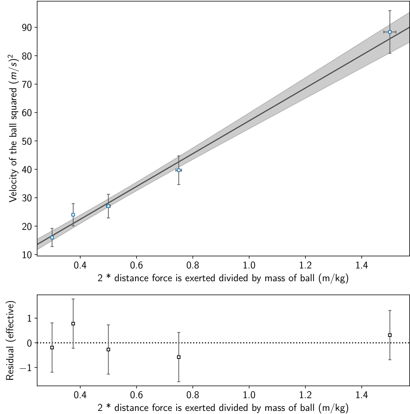
Finding Force exerted by the piston on the ball
