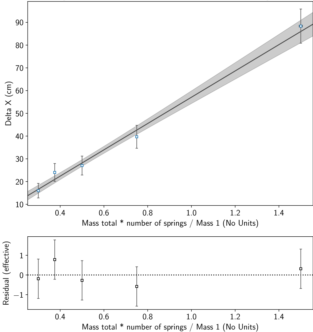
Graphing Delta X for the number of equivalent springs in series
