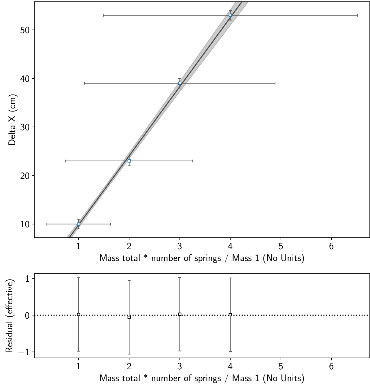
Finding Delta X for the number of equivalent springs in series
