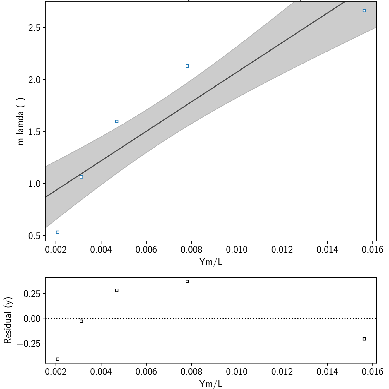
Green Laser (wavelength=532 nm)
