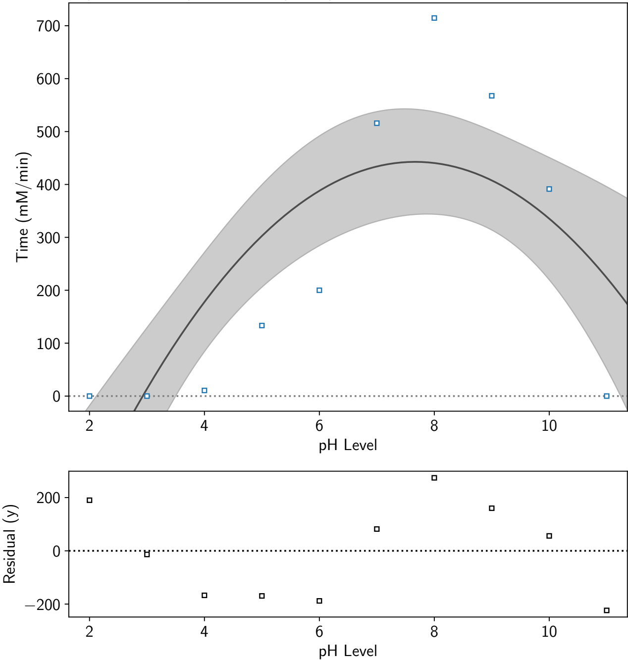
Trypsin Catalyzes the Hydrolysis of Proteins into Amino Acids
