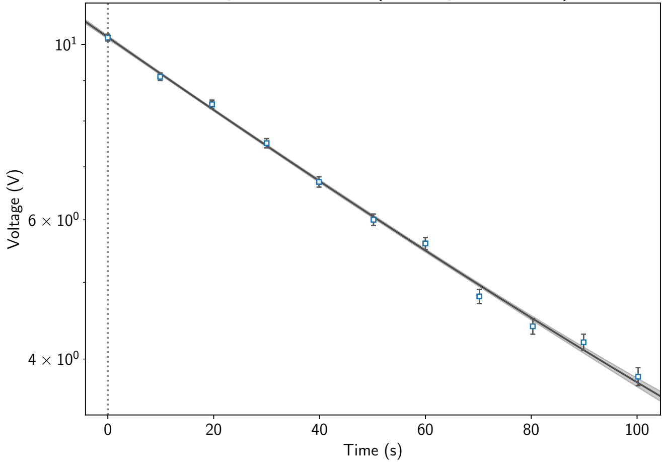
Voltage Versus Time (Semilogarithmic Fit)
