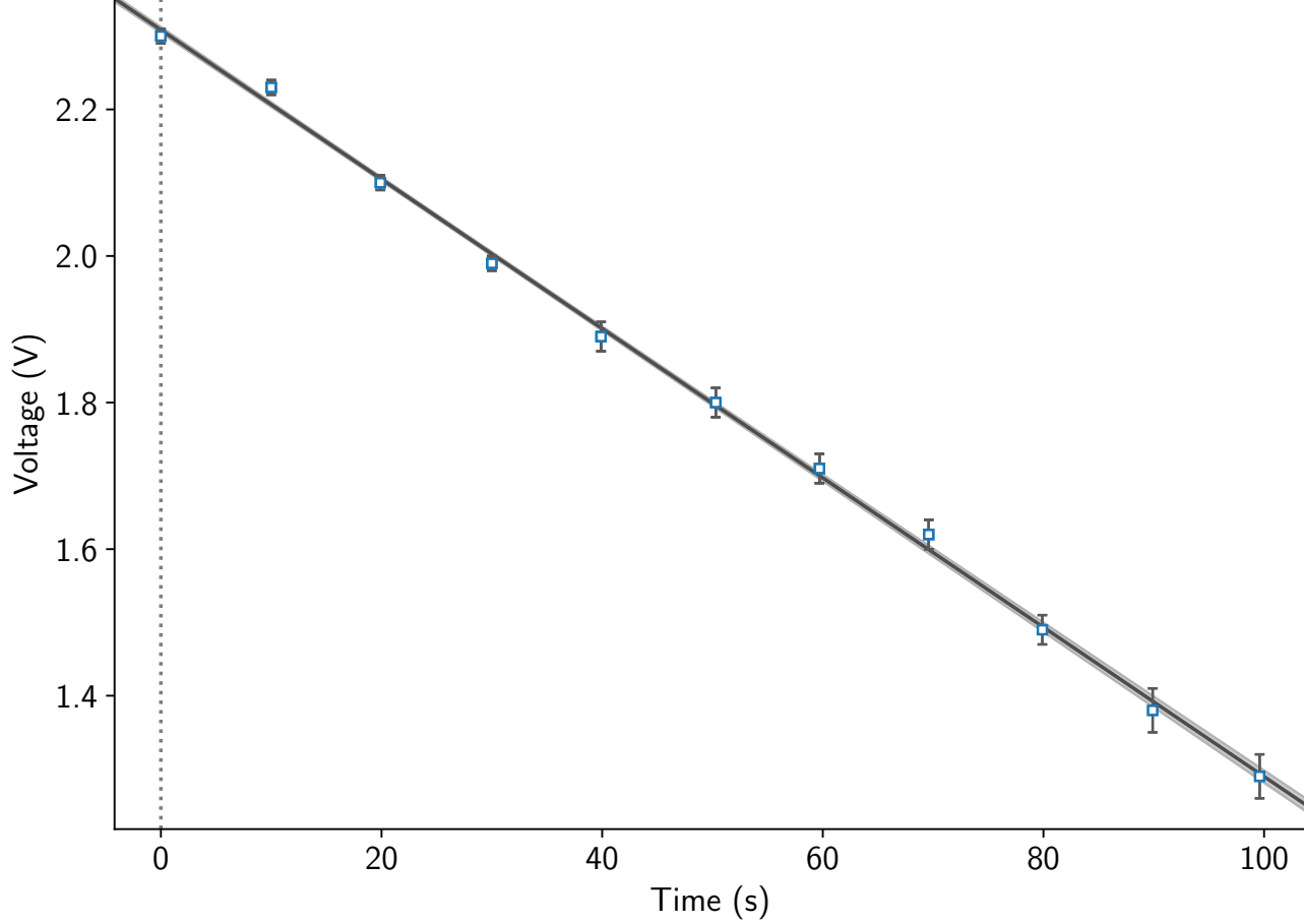
Voltage Versus Time (Linear Fit) - Converted
