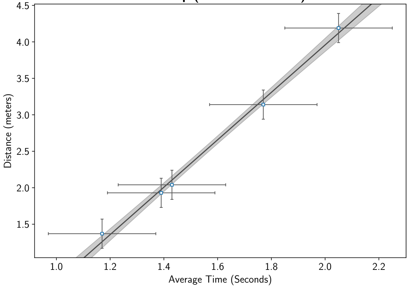
Ball Drop (Distance Vs Time)
