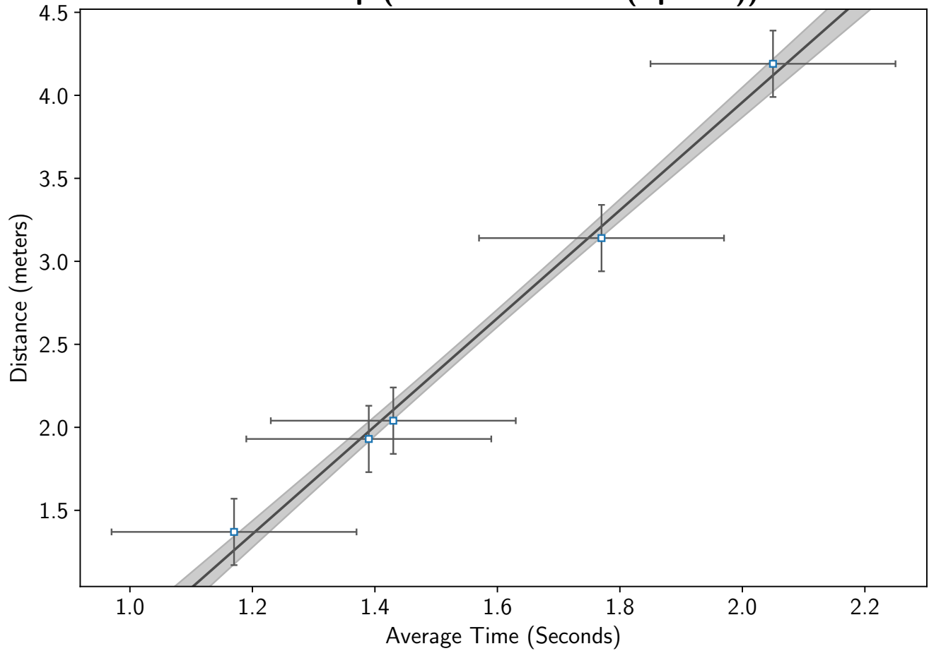
Ball Drop (Distance Vs Time(squared))
