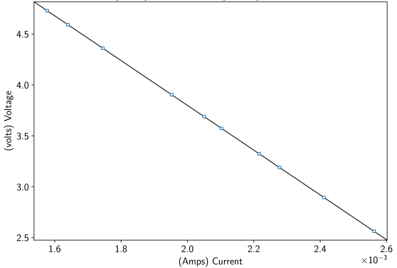
(volts) Voltage vs. (Amps) Current
