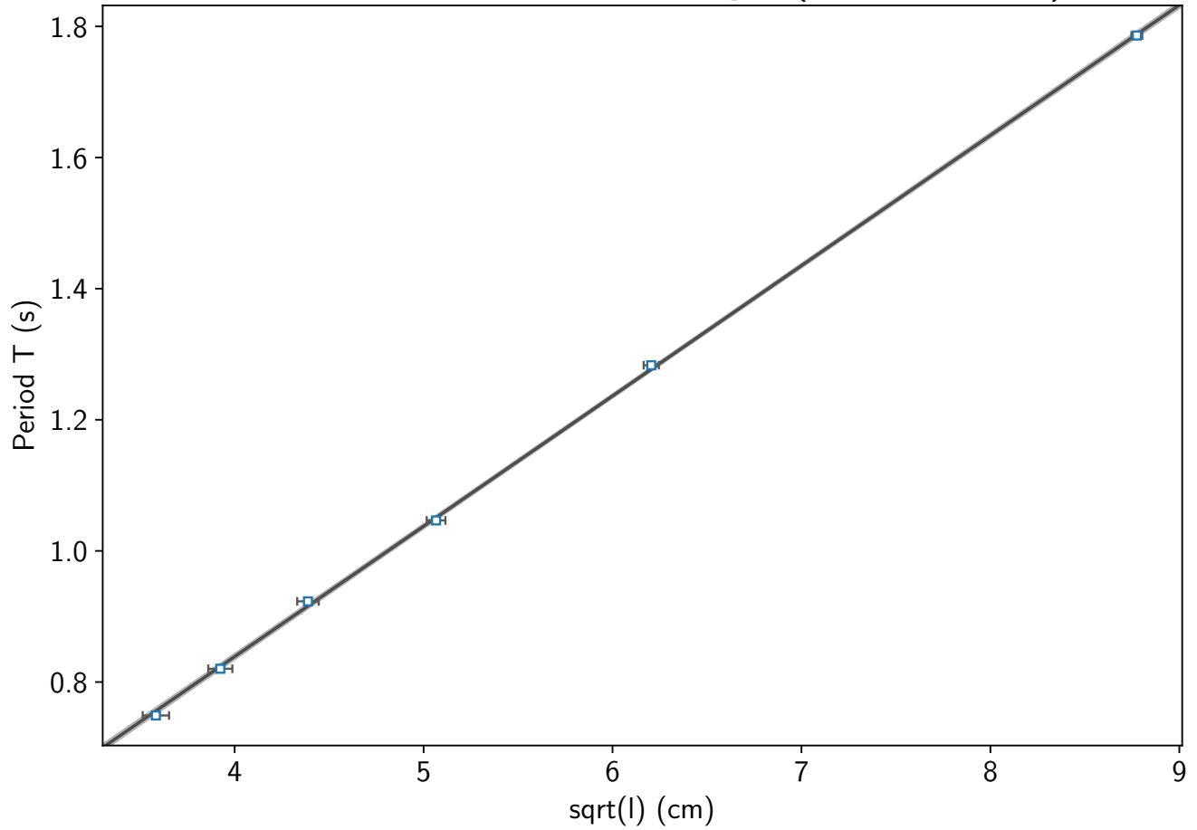
Period vs. Square Root of Length (Linearization 1)
