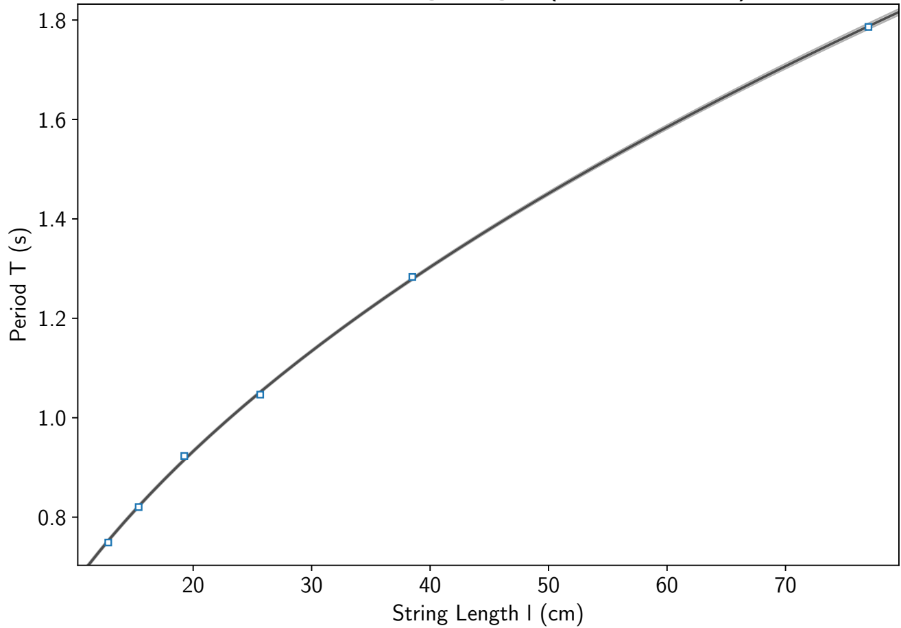
Period vs. String Length (Power Law Fit)
