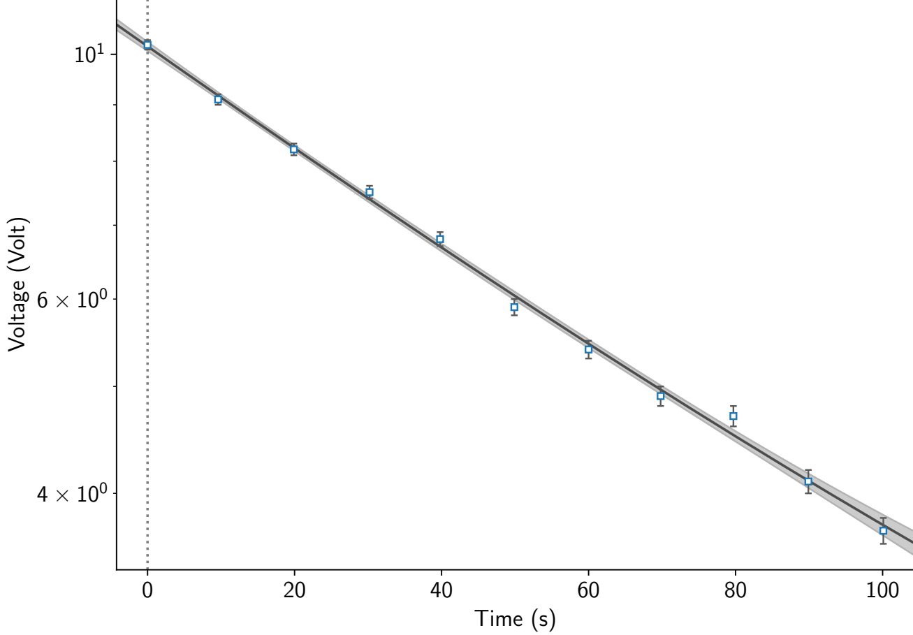
Exponential Fit Voltage (Volt) vs Time (s) Graph
