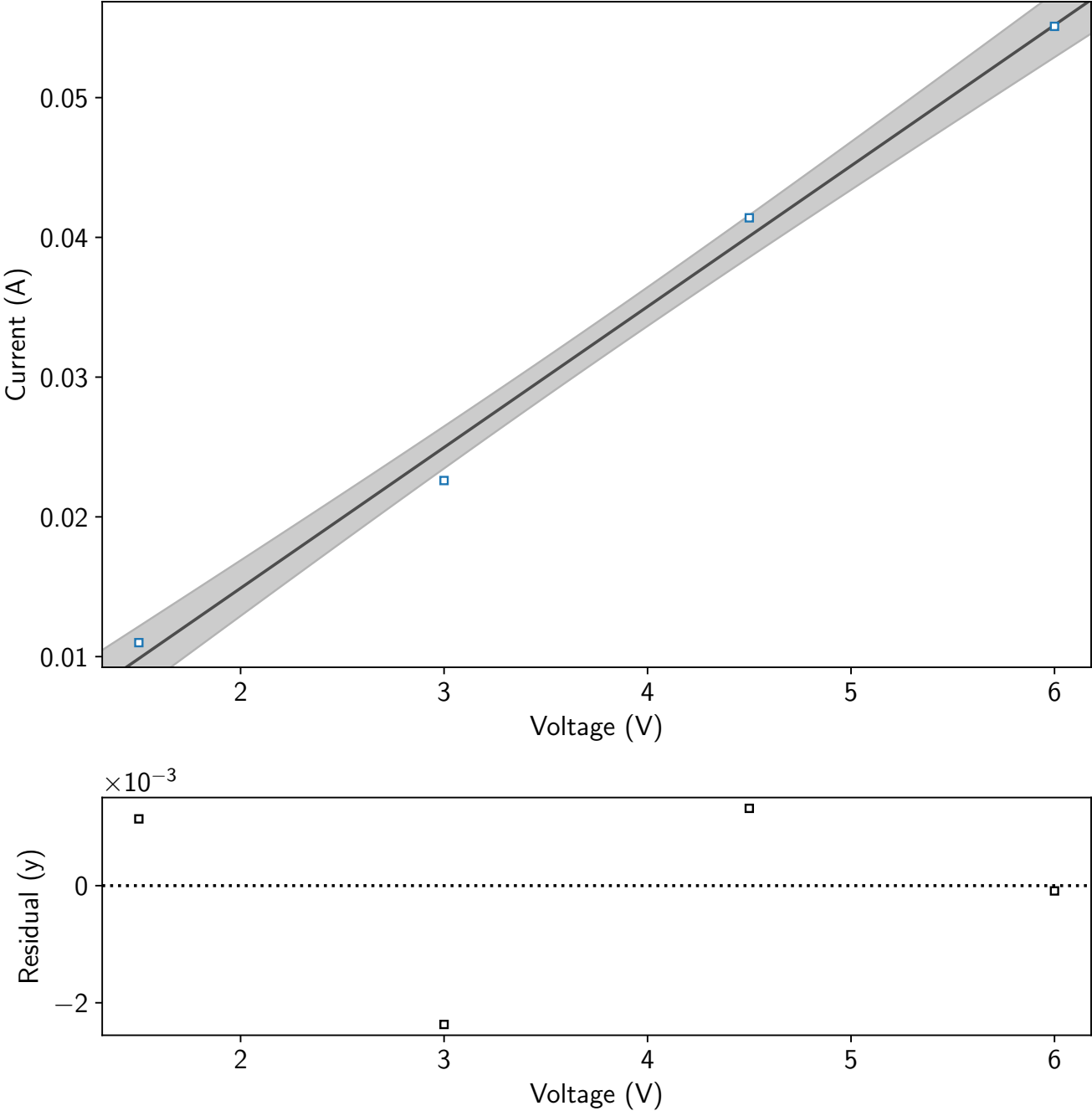
Ohm's Law (100 Ohm Resistor)
