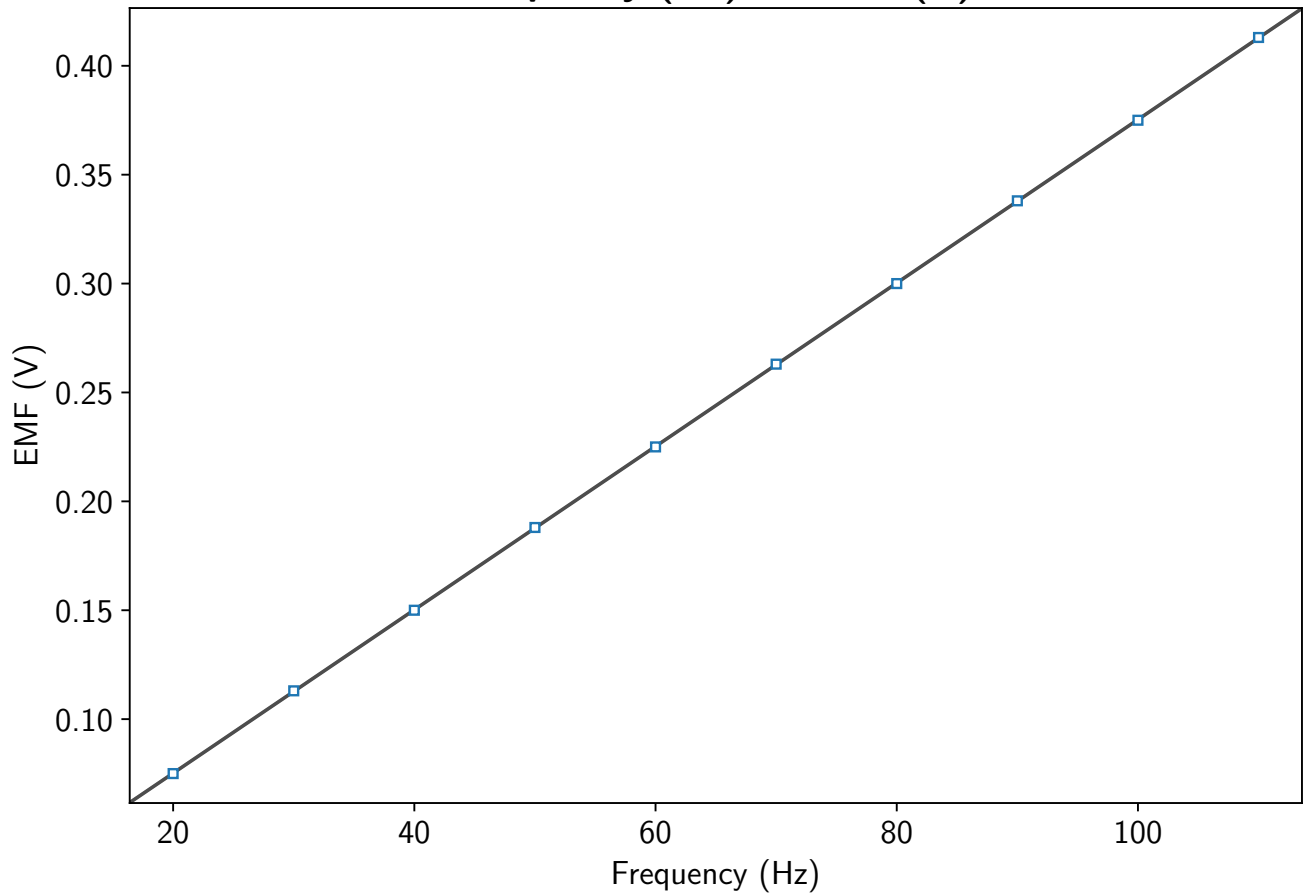
Frequency (Hz) vs EMF (V)
