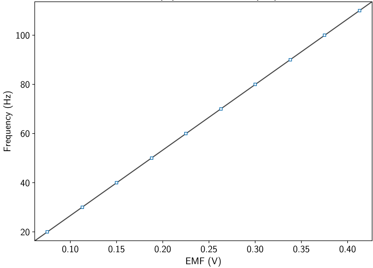
EMF (V) vs Frequency (Hz)
