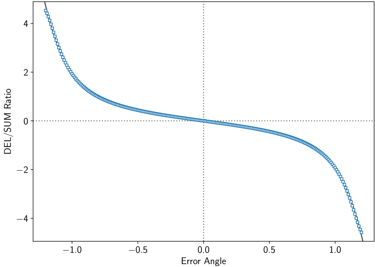
Monopulse Error Curve
