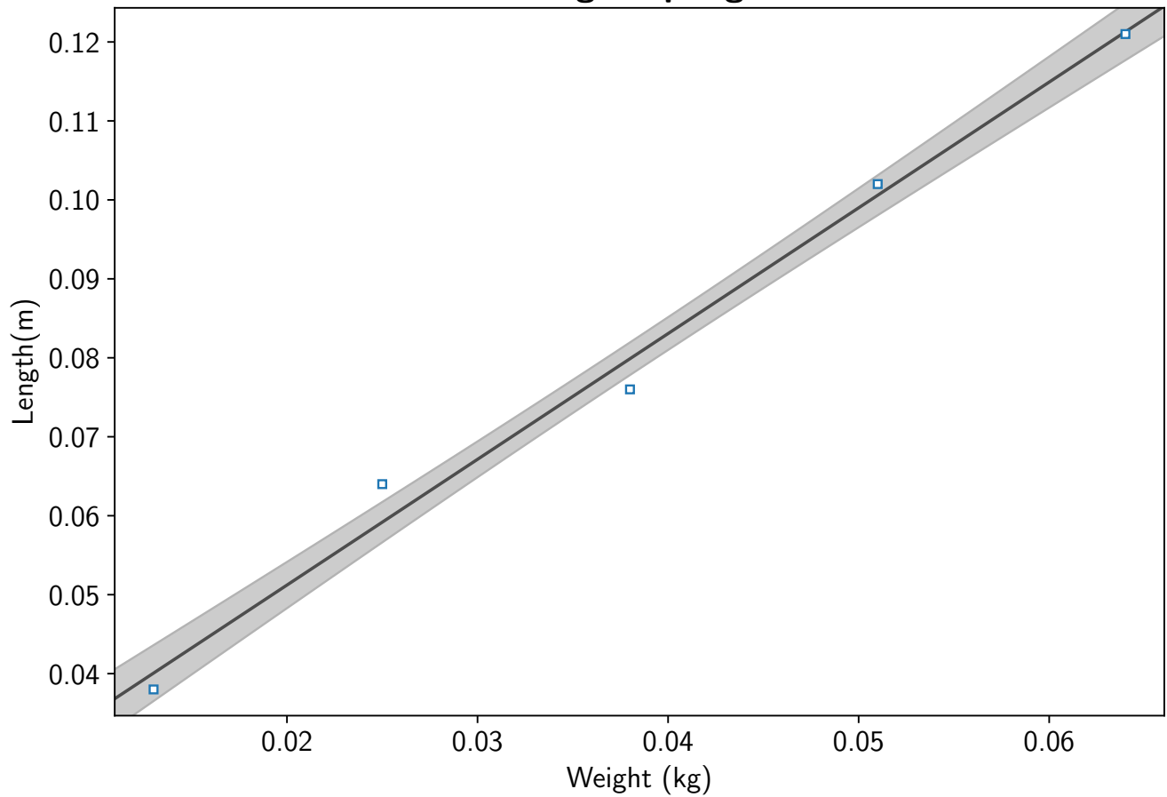
Mass vs Length Spring Constant
