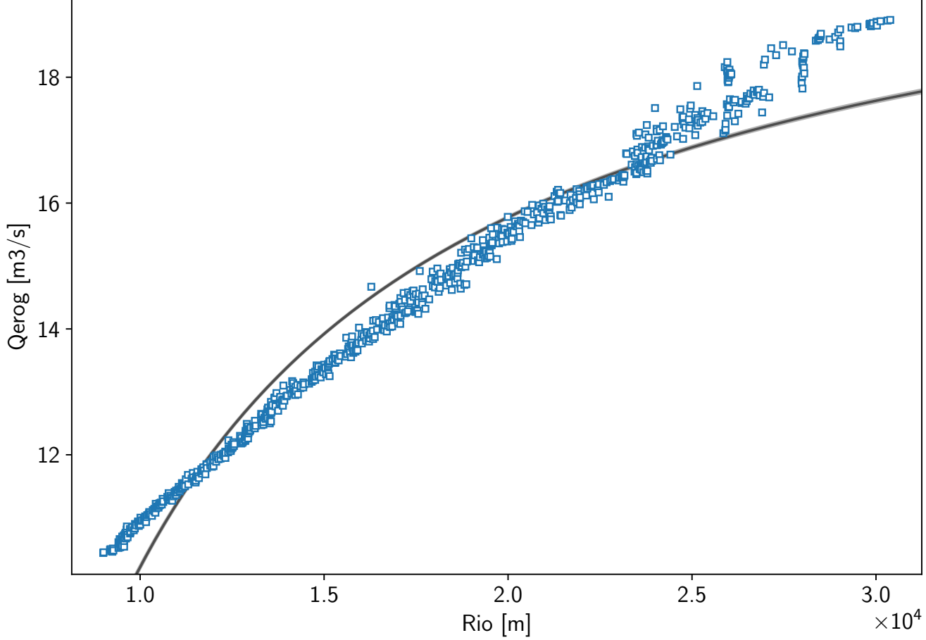
Rio vs Qerog - Tramo 2 (9000 - 30000 m3/s)
