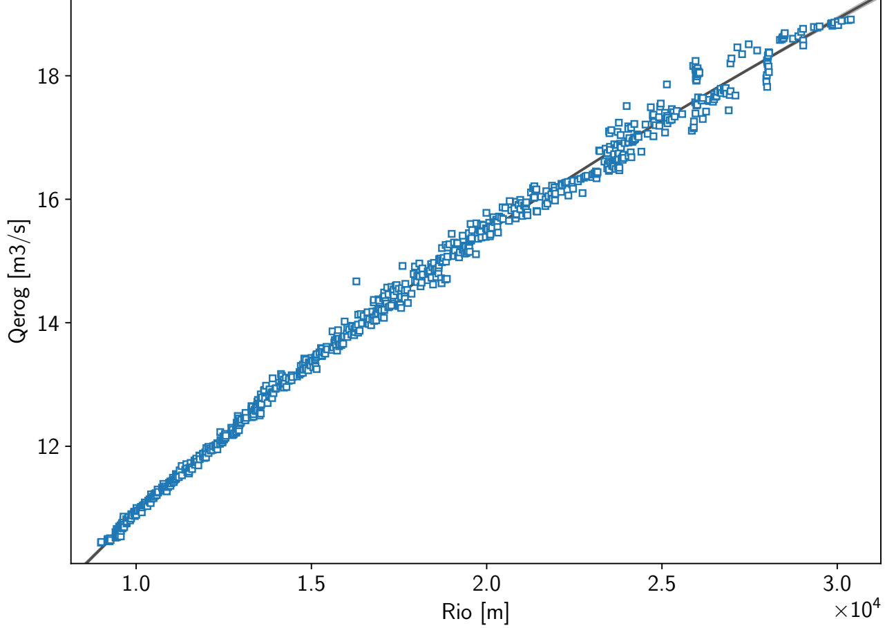
Rio vs Qerog - Tramo 2 (9000 - 30000 m3/s)
