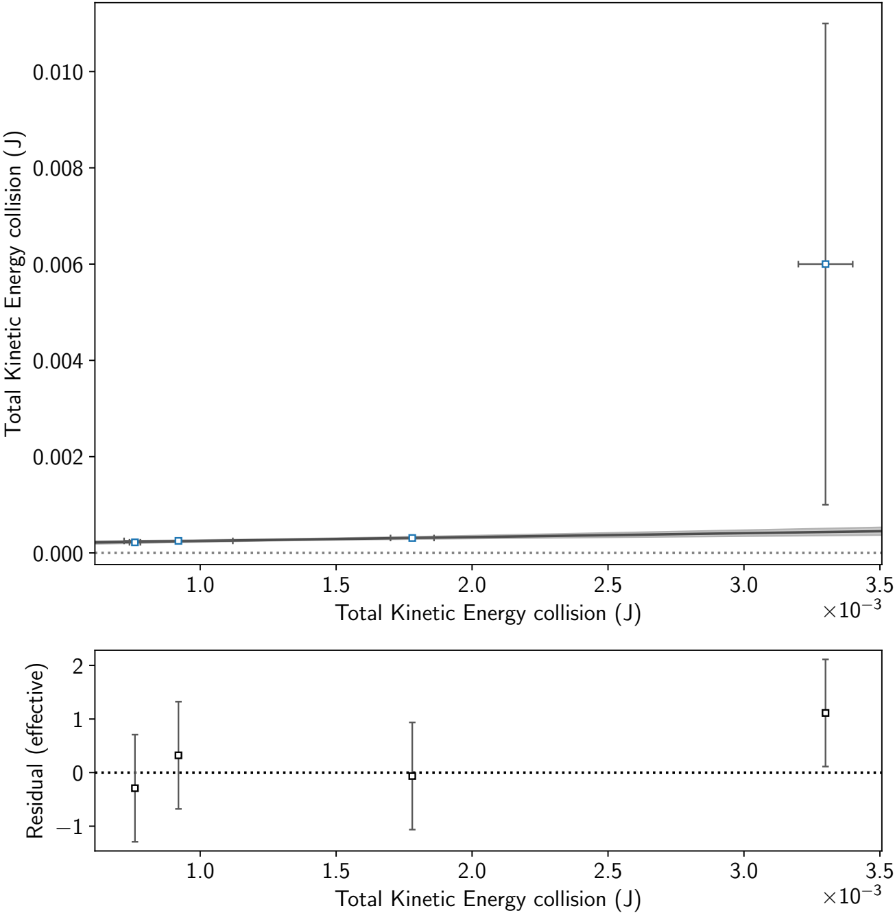
Total Kinetic Energy before vs. after the collision
