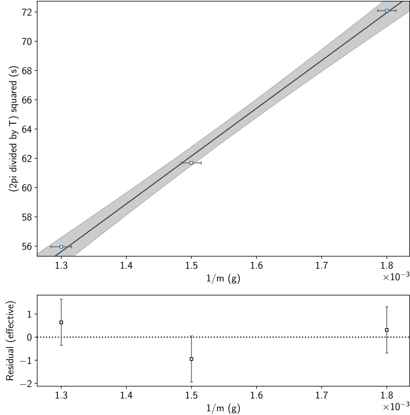
Spring Constant with 3 Springs in Series
