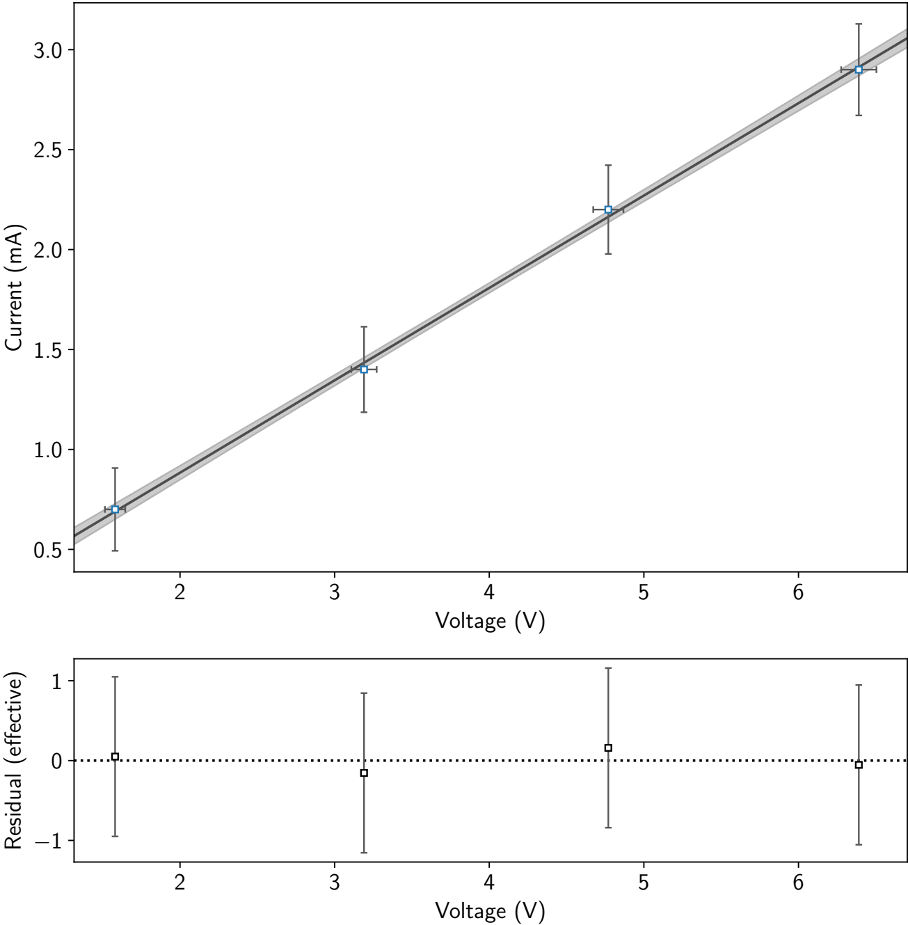
Current vs. Voltage (2200 Ohm)
