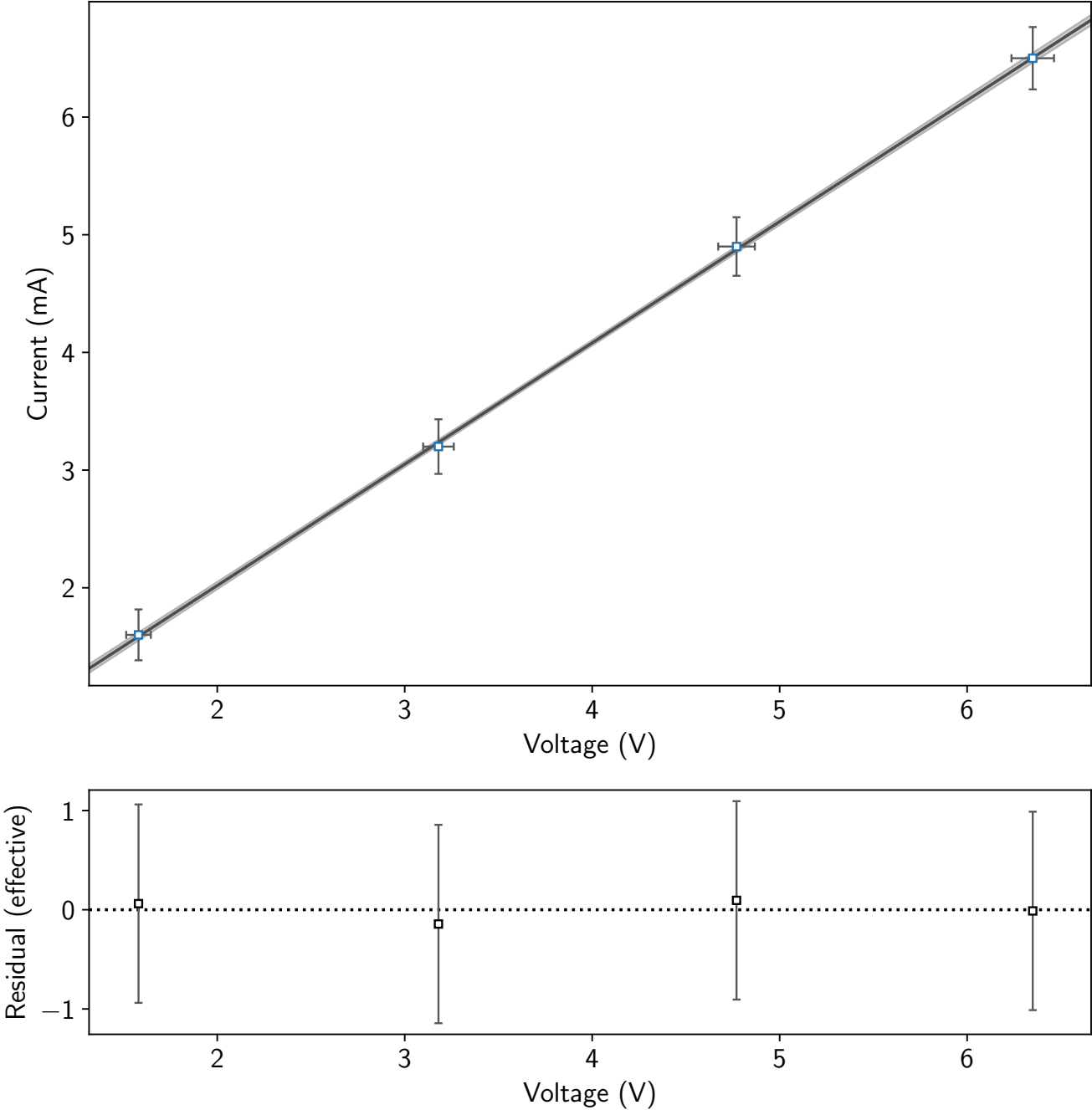
Current vs. Voltage (1000 Ohm)
