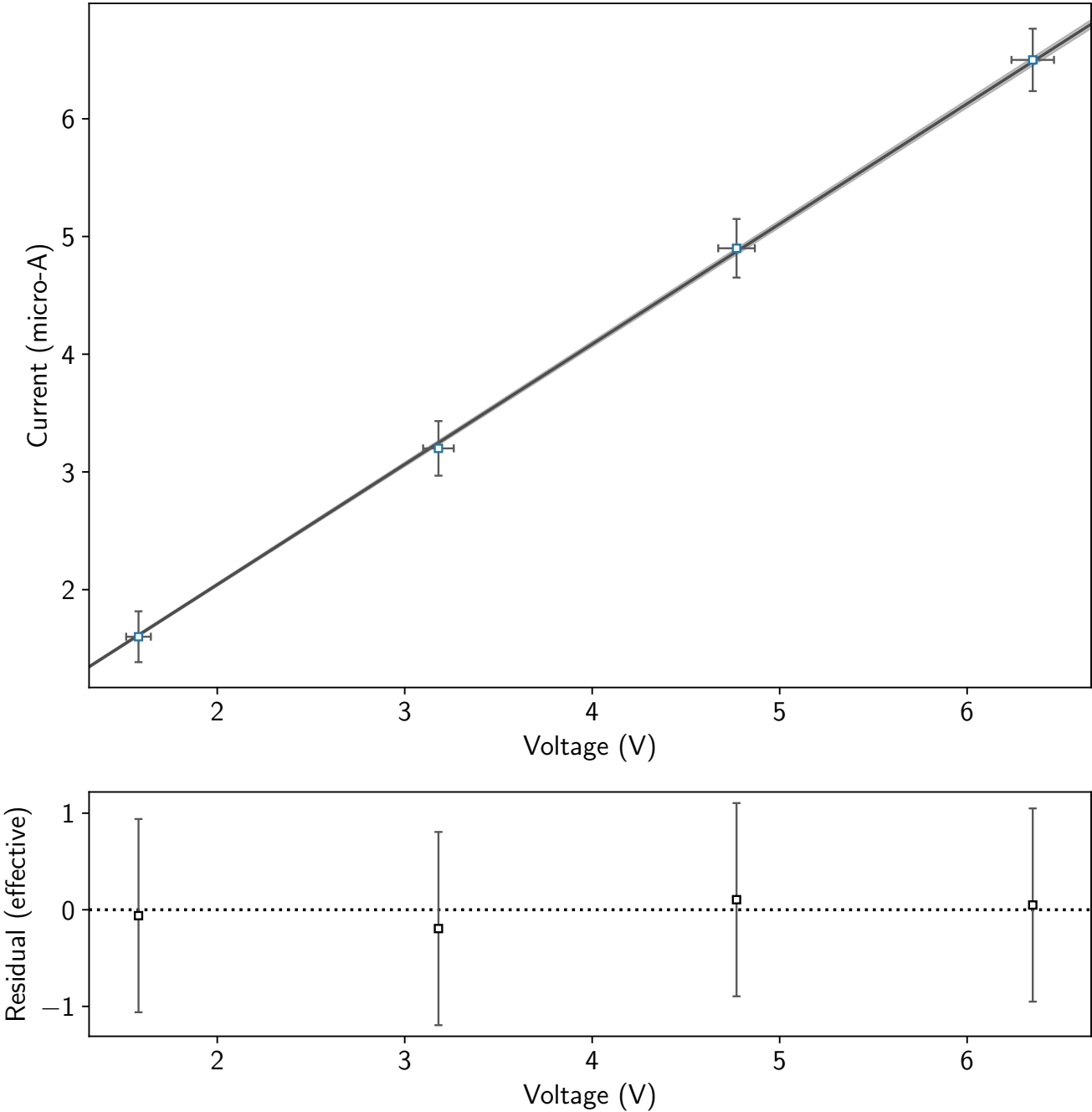
Current vs. Voltage (10000 Ohm)
