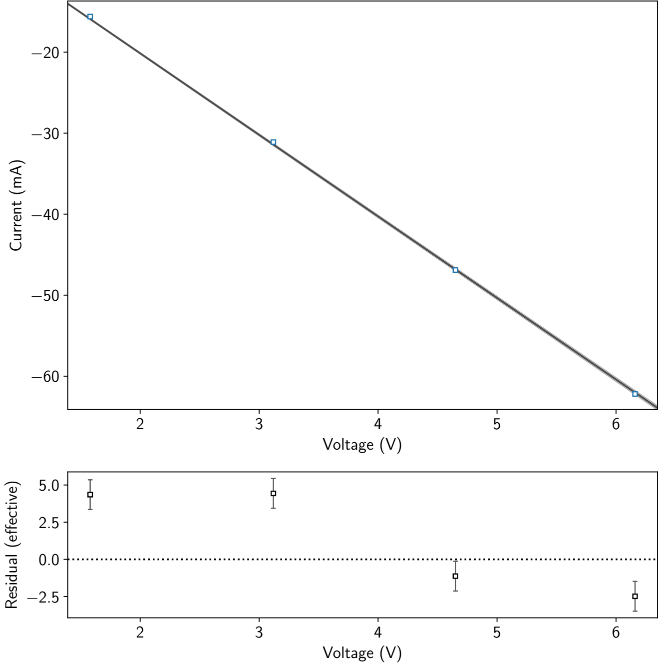
Current vs. Voltage (100 Ohm)
