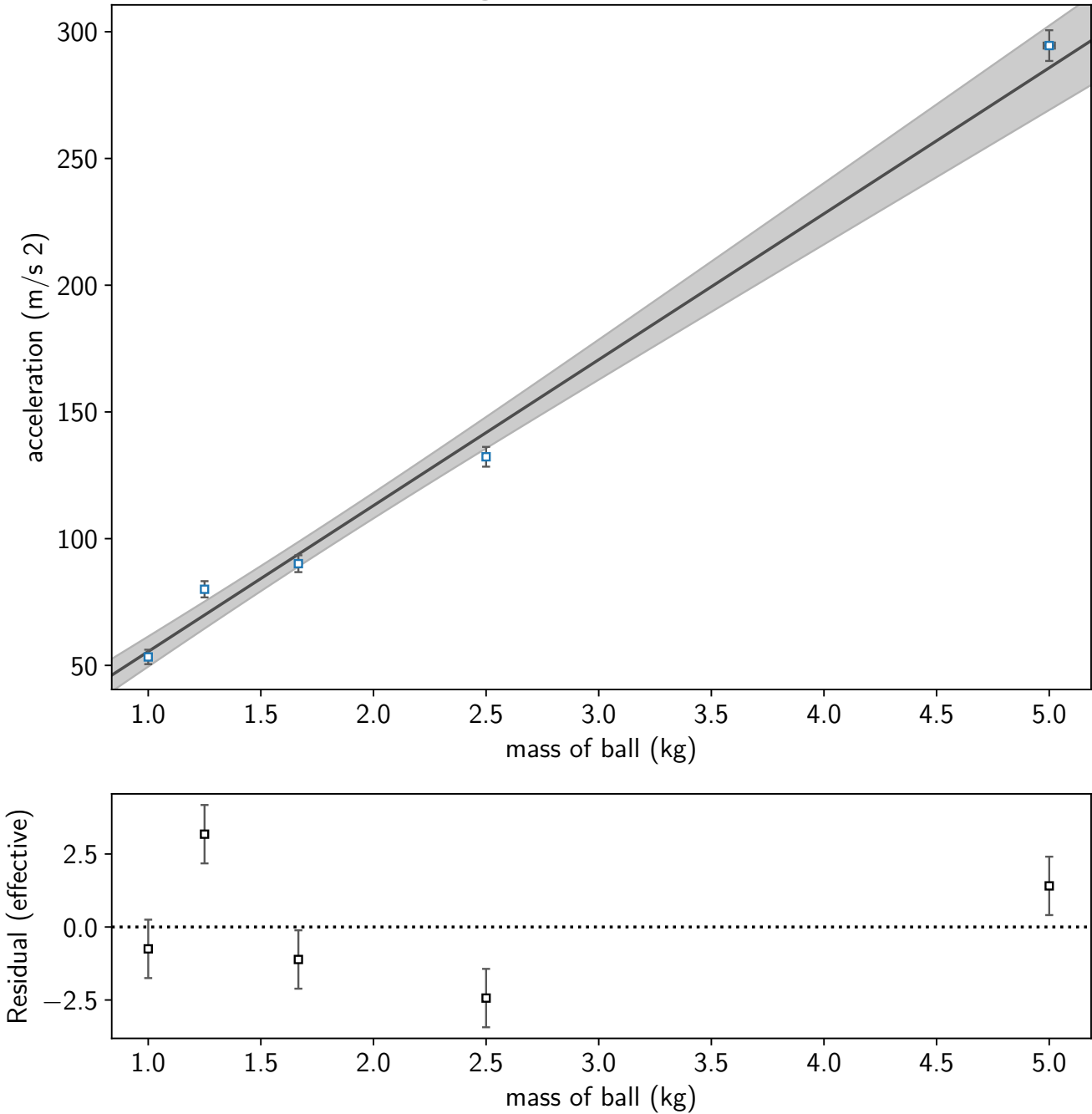
Determining Minimum Force of Piston
