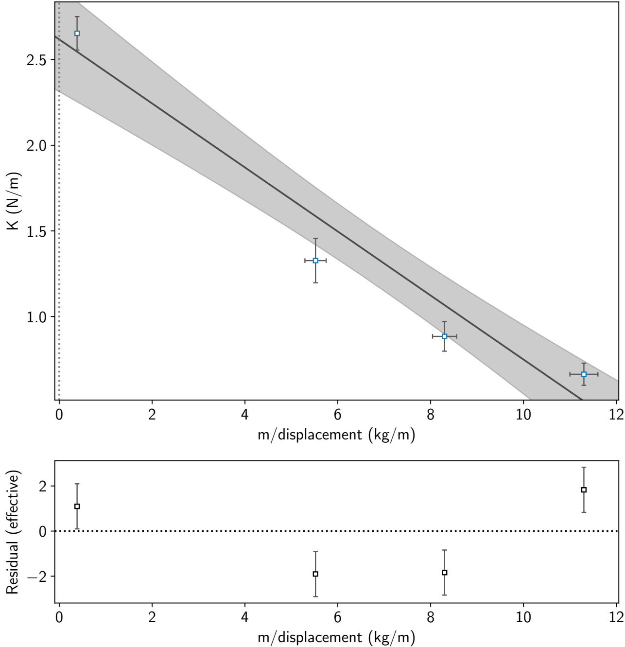
Determining Gravity of using a series of springs
