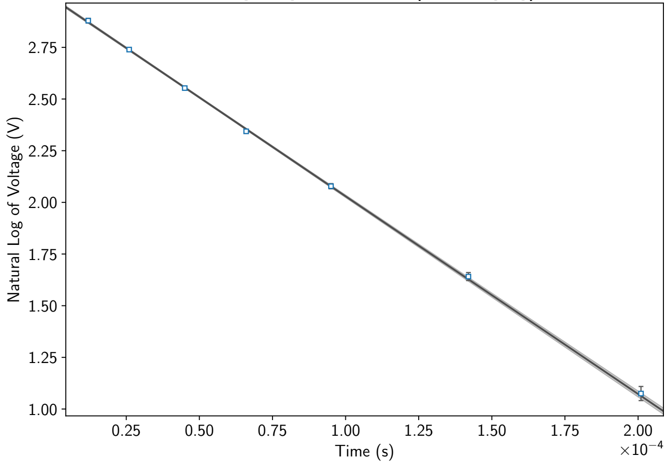
Voltage Signal vs Time (Discharging)
