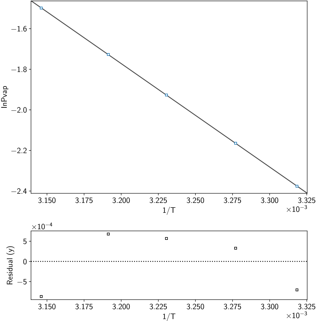
InPvap vs The Reciprocal of Absolute Temperature
