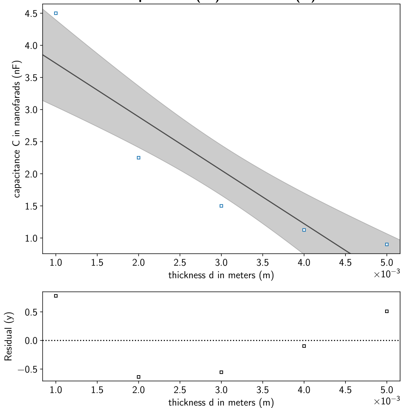
capacitance (nF) vs thickness (m)
