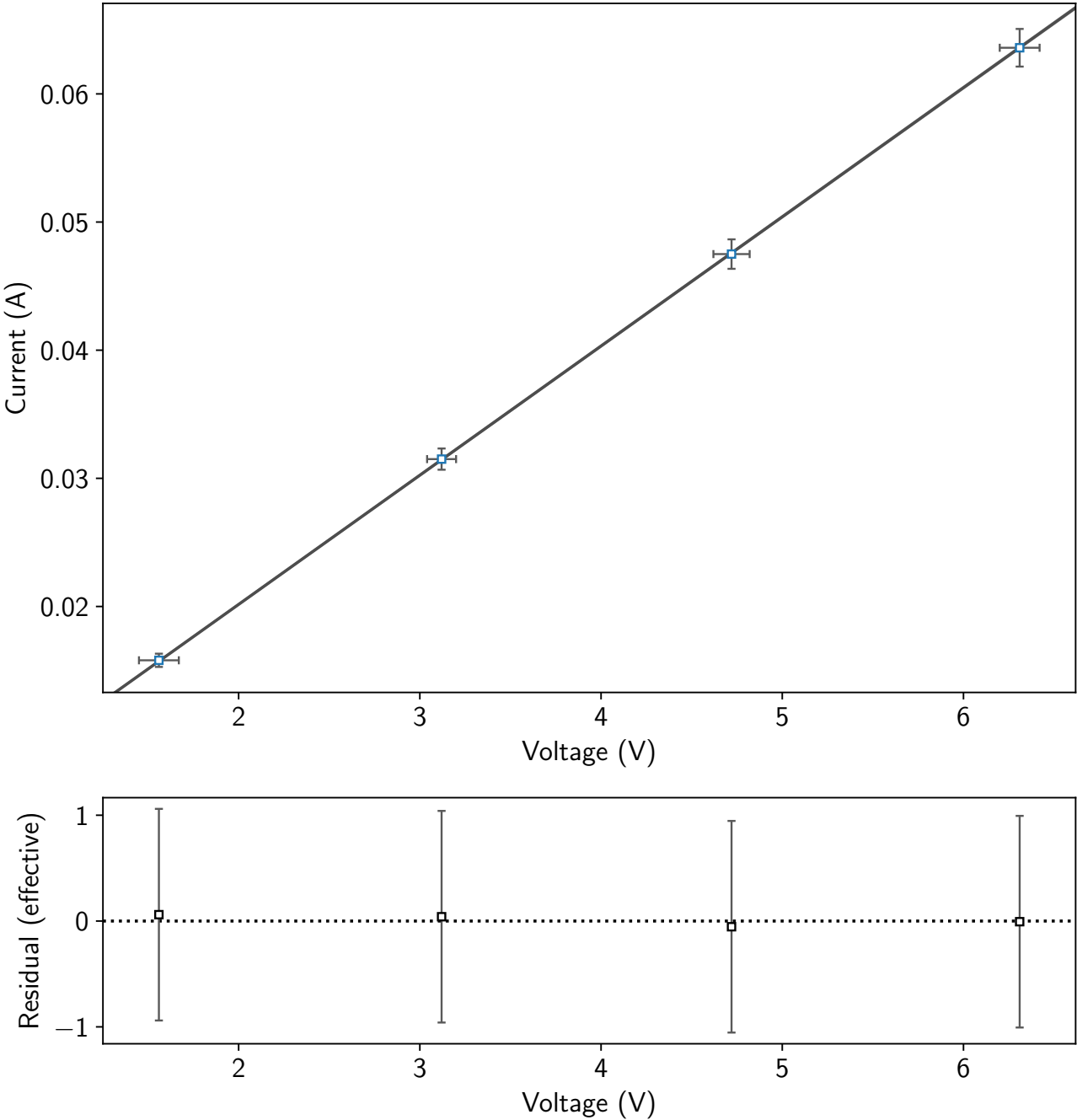
100 Ohm Resistor: Current (A) as a Function of Voltage (V)
