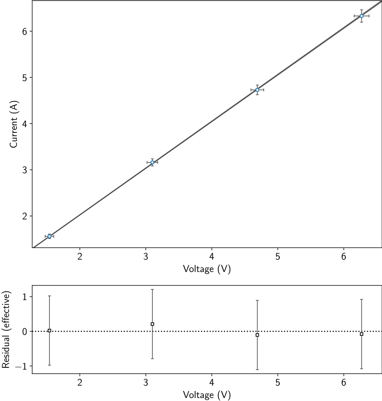
10000 Ohm Resistor: Current (A) as a Function of Voltage (V)
