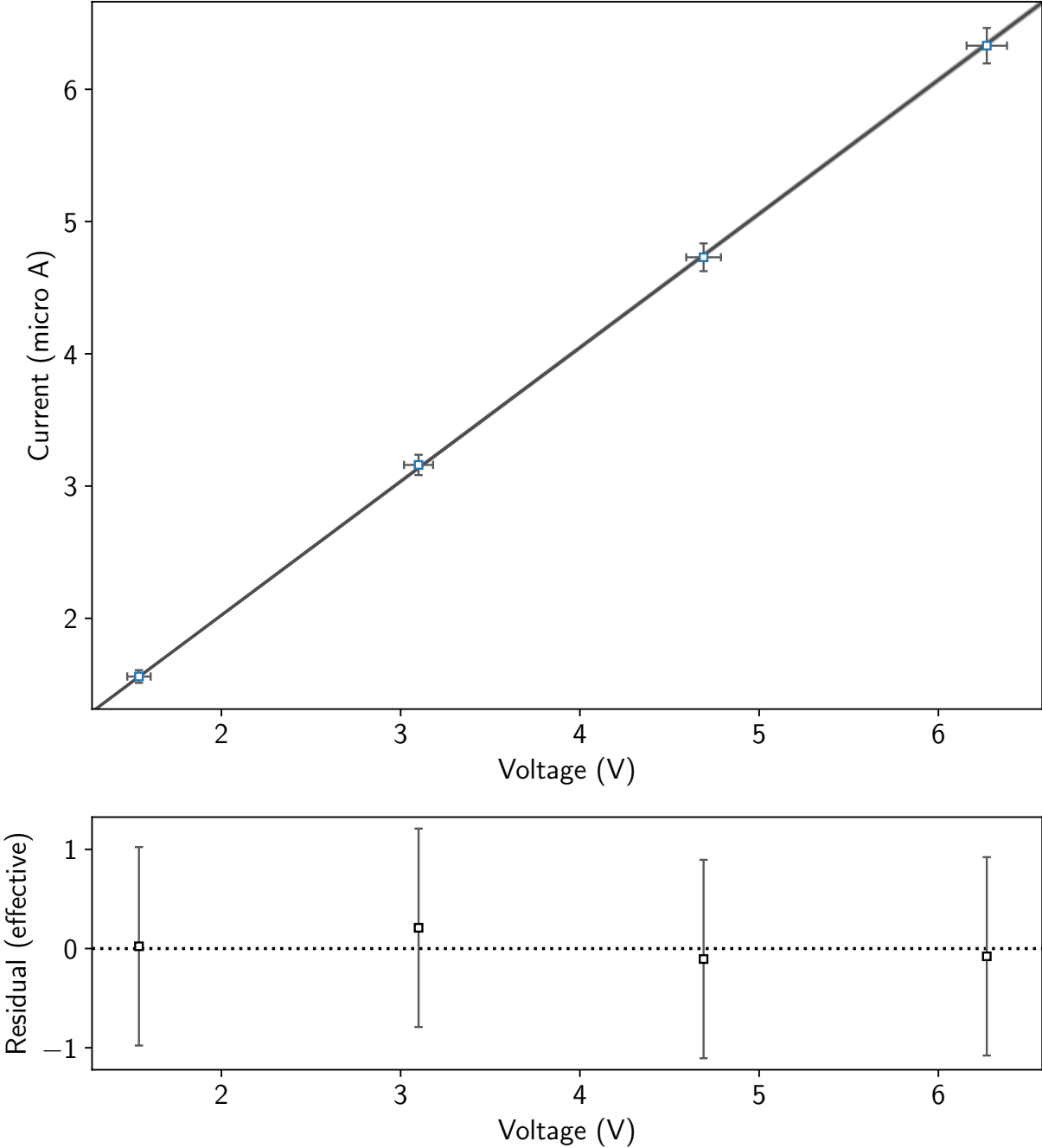
10000 Ohm Resistor: Current (micro A) as a Function of Voltage (V)
