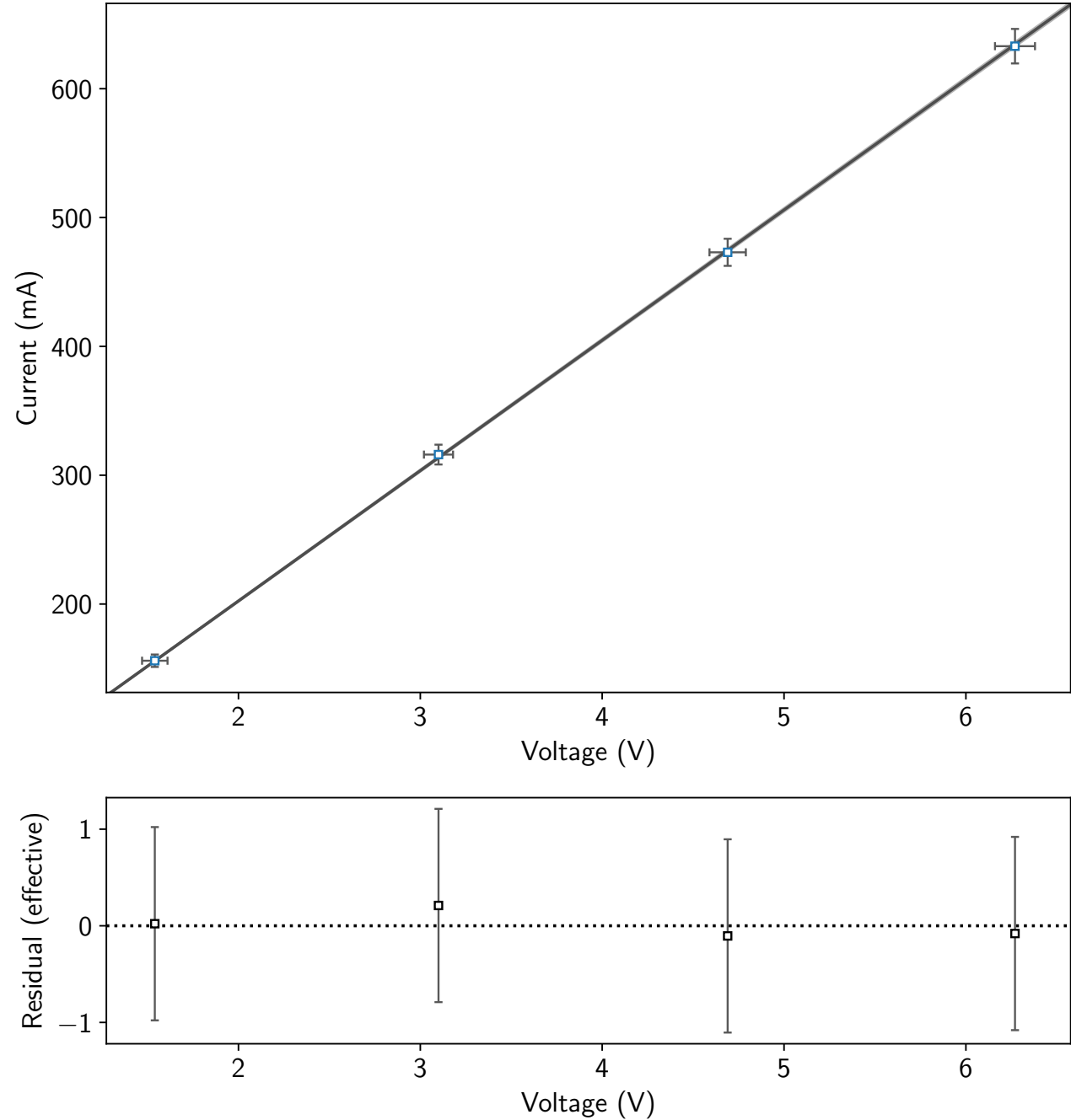
2200 Ohm Resistor: Current (mA) as a Function of Voltage (V)
