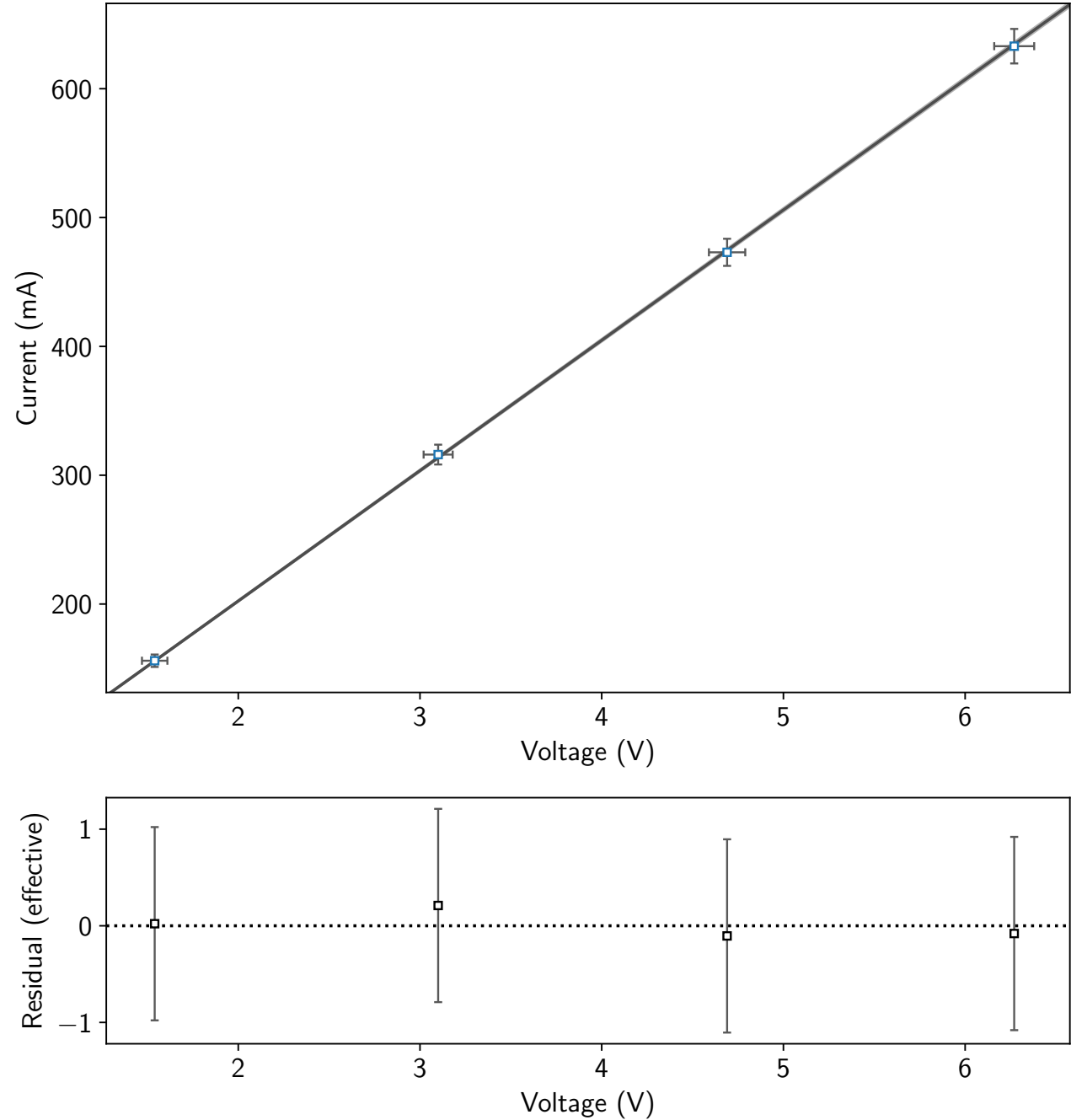
1000 Ohm Resistor: Current (mA) as a Function of Voltage (V)
