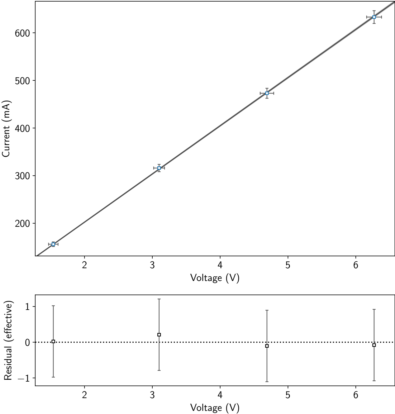
100 Ohm Resistor: Current (mA) as a Function of Voltage (V)
