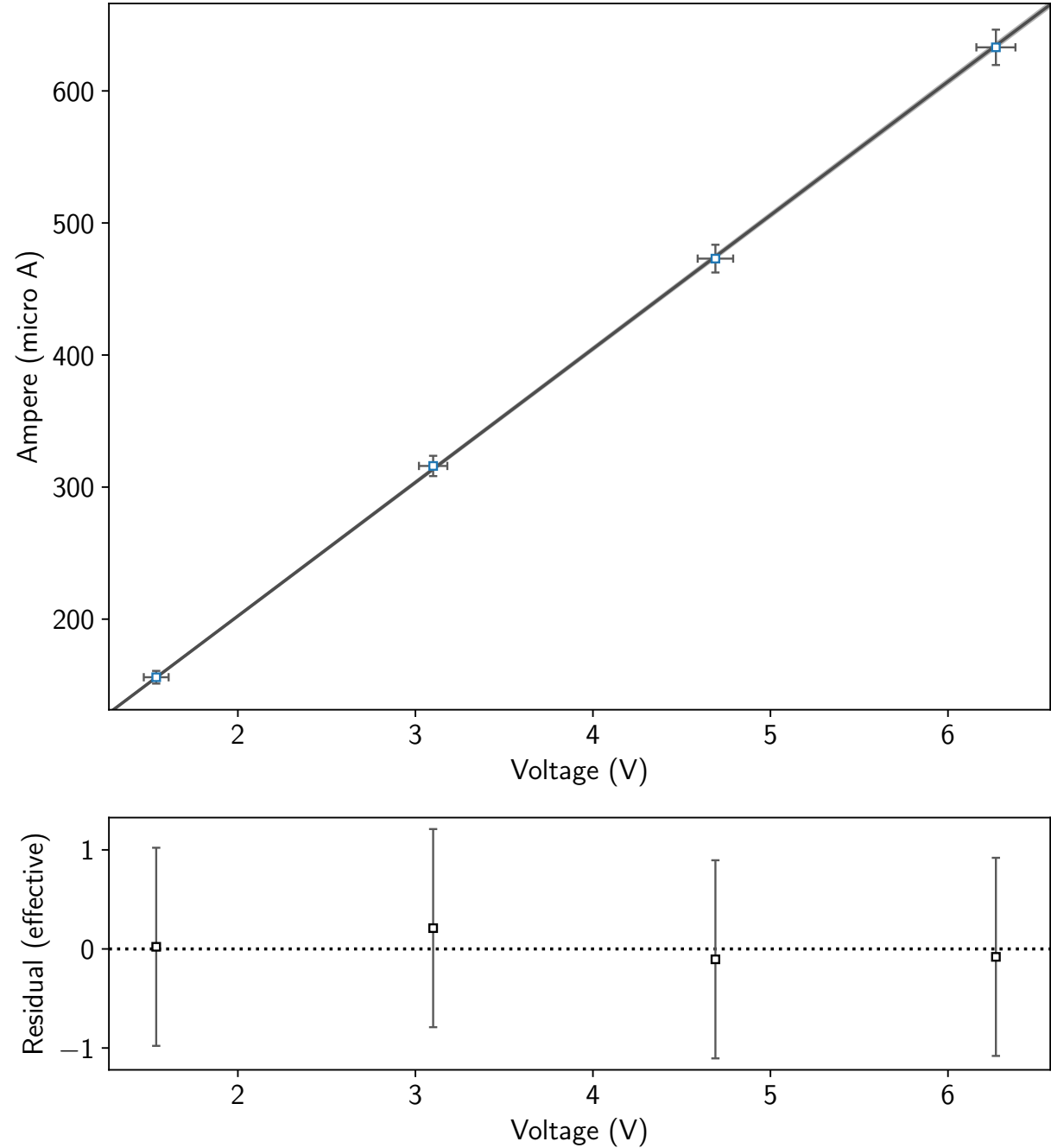
10000 Ohm Resistor: Ampere (micro A) as a Function of Voltage (V)
