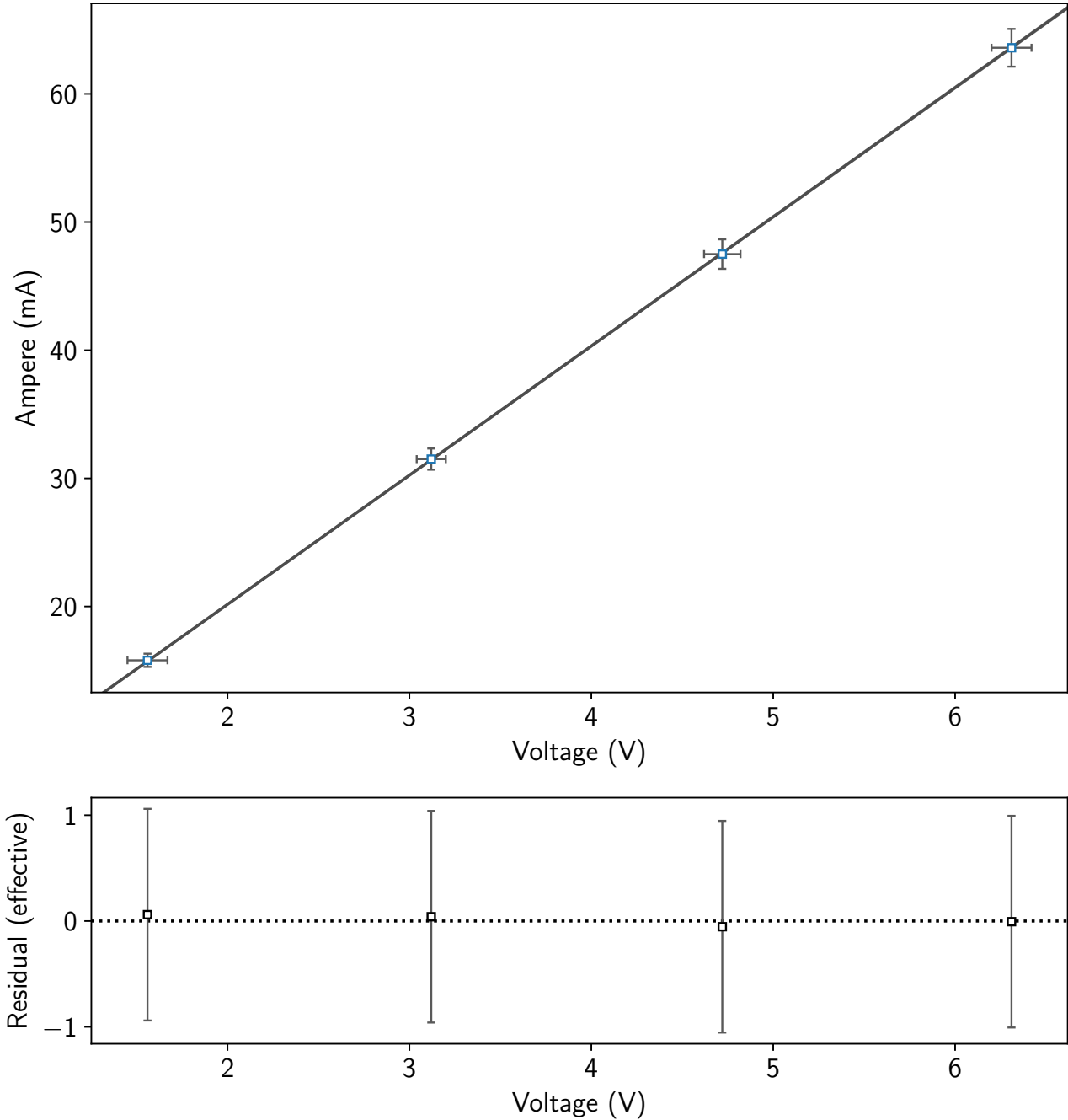
100 Ohm Resistor: Ampere (mA) as a Function of Voltage (V)
