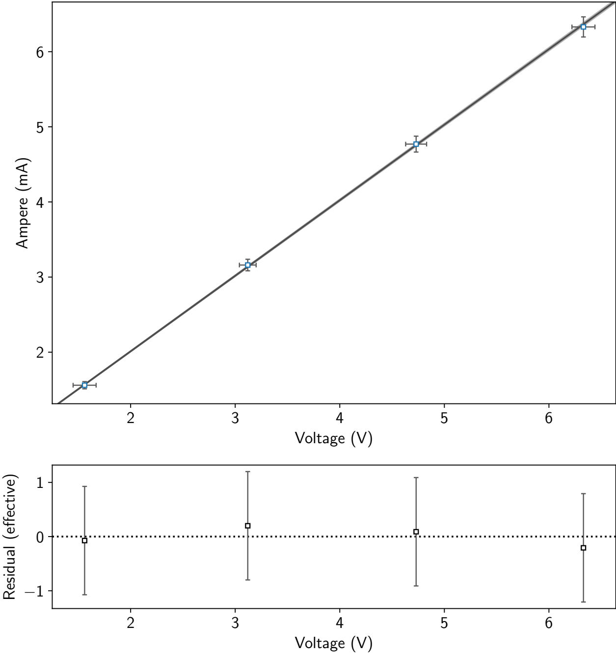
1000 Ohm Resistor: Ampere (mA) as a Function of Voltage (V)
