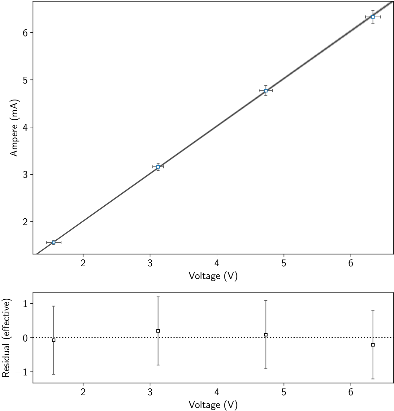
1000 Ohm Resistor: Ampere (A) as a Function of Voltage (V)
