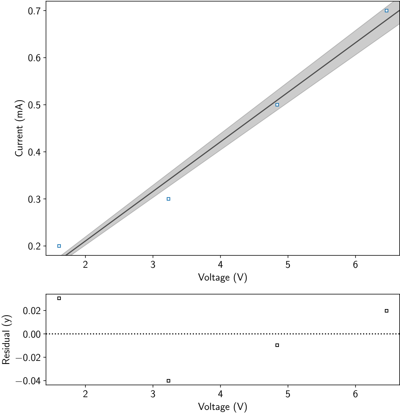
Current vs Voltage fot the 10000 Ohm Resistor
