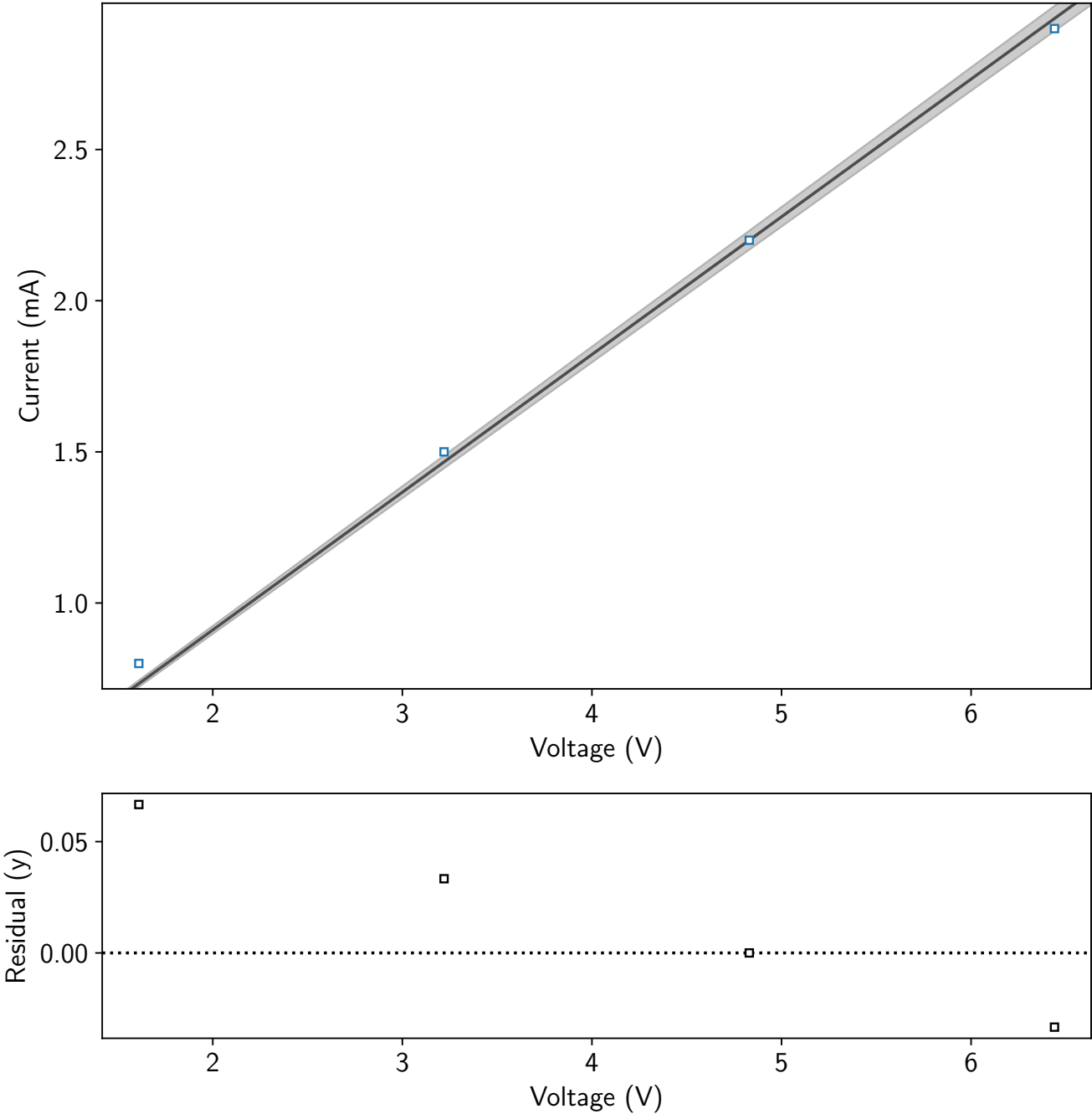
Current vs Voltage fot the 2200 Ohm Resistor
