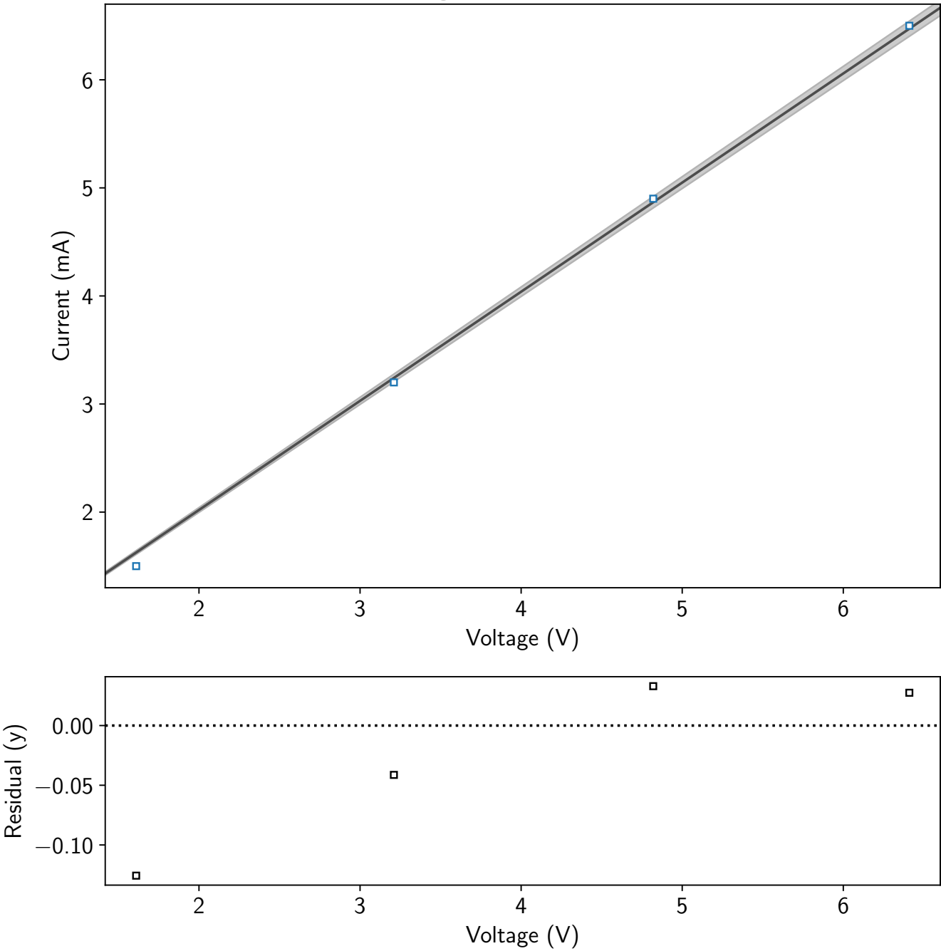
Current vs Voltage fot the 1000 Ohm Resistor
