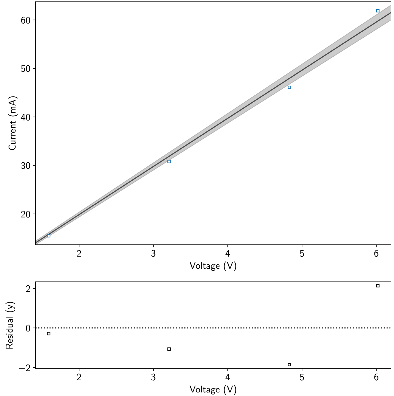
Current vs Voltage fot the 100 Ohm Resistor
