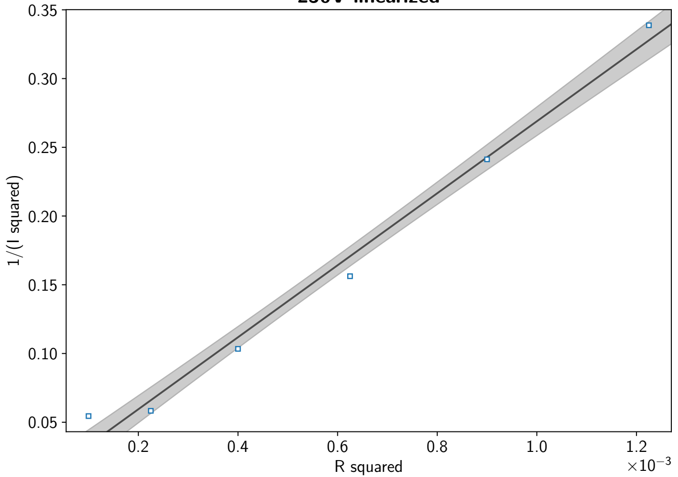
250V linearized
