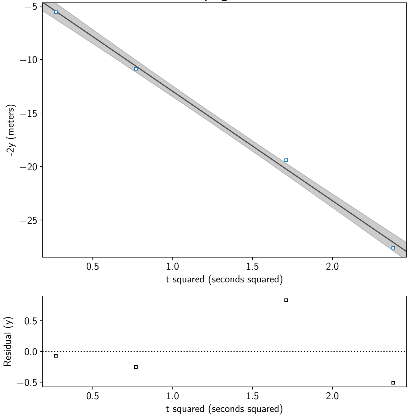
Ball Drop: g calculation
