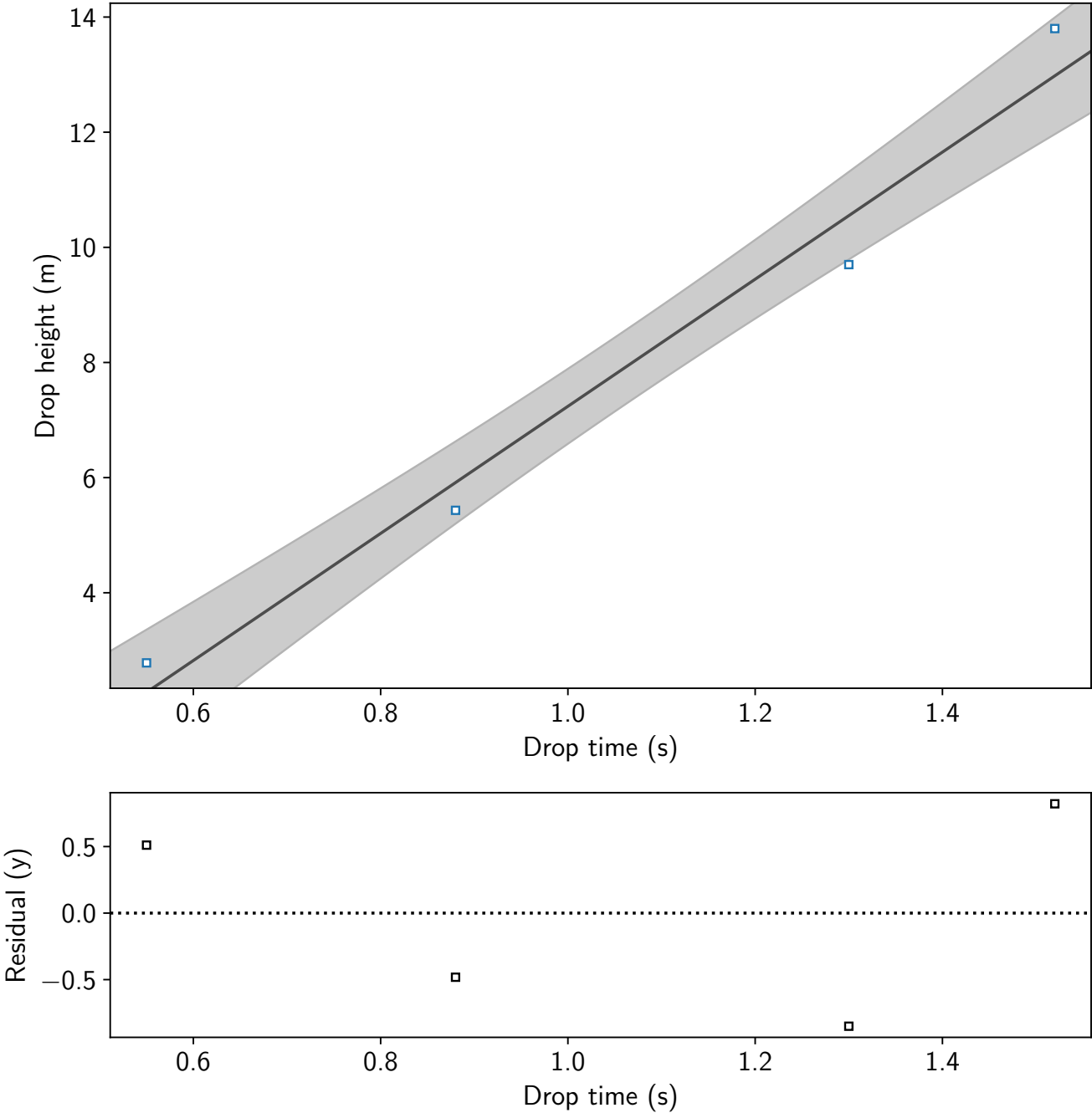
Ball Drop time vs Ball Drop height
