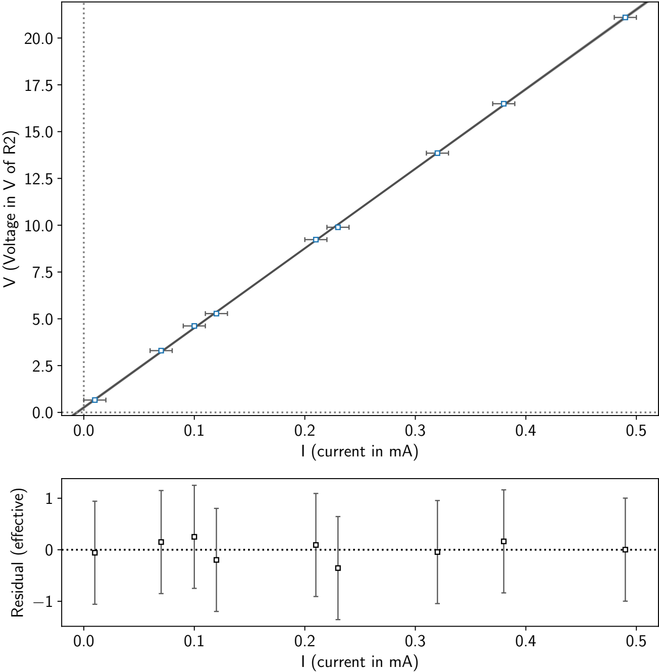
Ohm's Law With Double Resistor
